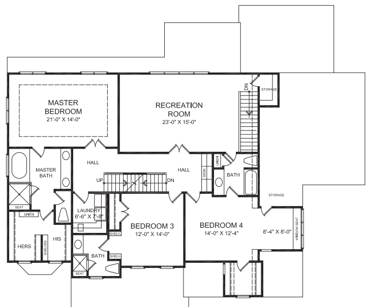
SECOND FLOOR
